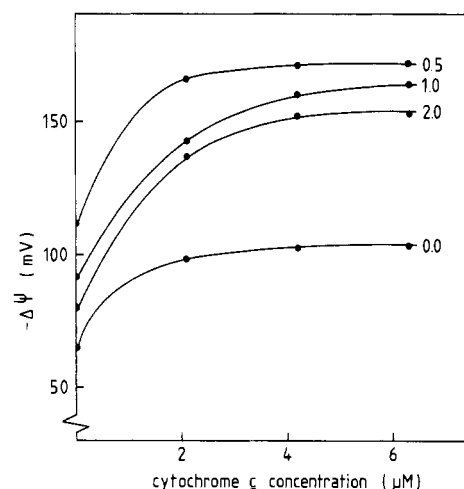
FIGURE 10: Optimization of the reconstituted pump at pH 7.0 with respect to protonmotive force generation in RC/LHI/LHII liposomes. \Delta\psi measurements were performed at pH 7.0 under standard conditions as described under Experimental Procedures. The numbers in the figure indicate the concentration of ascorbate in millimolar.
