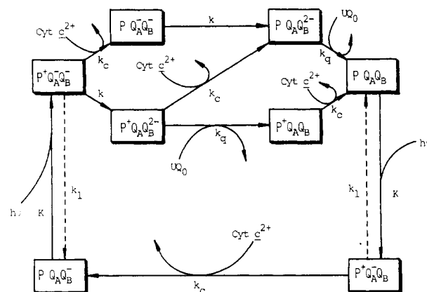
FIGURE 13: Simplified scheme of electron transfer in a suspension of RC's, cytochrome c 2+ , and UQ 0 . Steps in which cytochrome c 2+ , UQ 0 , or photons are involved have been modeled as second-order reactions. Symbols for first- or second-order reaction constants are indicated. Their approximate values are the following (from Table I): k , 800 s -1 ; k_c , 4 \times 10^8 \text{ M}^{-1}\text{s}^{-1} ; k_q , 1 \times 10^7 \text{ M}^{-1}\text{s}^{-1} . The cytochrome c 2+ concentration was varied from 0.25 to 50 μM, and the UQ 0 concentration was 400 μM. Under the conditions used, the rate of re-reduction of cytochrome c by UQ 0 H 2 is negligible as could be concluded from absorption measurements after turning off actinic light (an example of this type of measurement is shown in Figure 9). Symbols: P, primary electron donor of the RC's (special pair of bacteriochlorophyll); Q A and Q B , RC-associated primary and secondary electron-accepting quinone, respectively; h\nu , photon.
